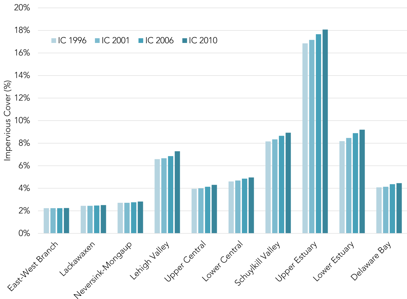
Figure 1.4.4 Percent impervious cover trends for the watersheds of the Basin for the four time periods analyzed: 1996, 2001, 2006, and 2010.
