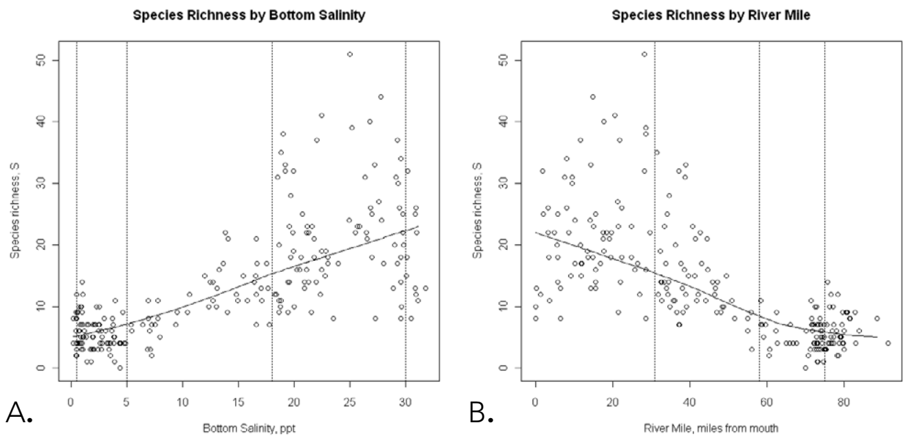
Figure 5.1.2 Patterns of benthic species diversity, comparing species richness versus A) bottom salinity and B) river mile.
