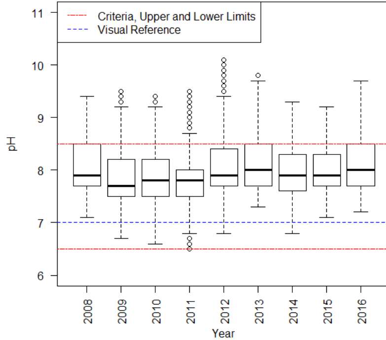
Figure 3.2.8 Instantaneous pH measurements by year, Delaware River at USGS 01463500, Trenton, 2008 through 2016.
