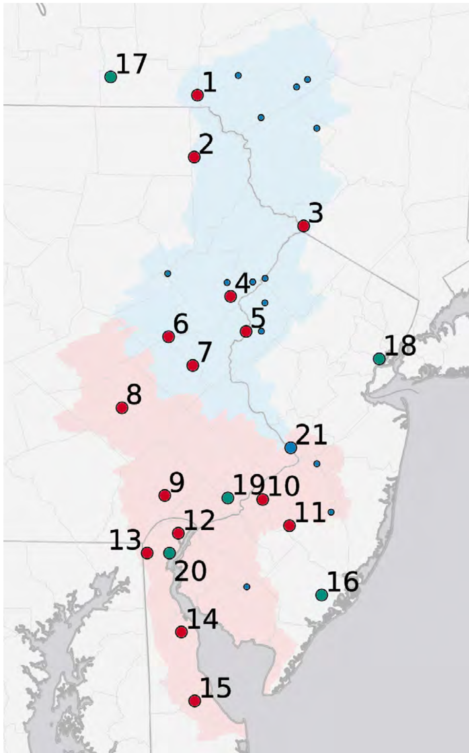
Figure 7.1.1 Location of meteorological and hydrological stations used in this analysis. Red dots (1–15) are the USHCN stations (section 7A); green dots (16–20) are the wind stations (7E); the blue dot (21) is the stream gauge at Trenton (7F).
