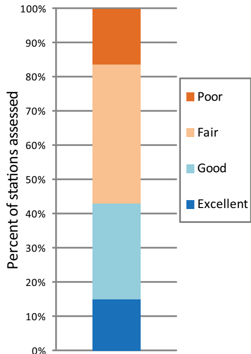
Figure 6.12.10 Bioassessment Station Data for New Jersey's Delaware River Basin, AMNET 3 Survey with 301 stations (2002-2007).
