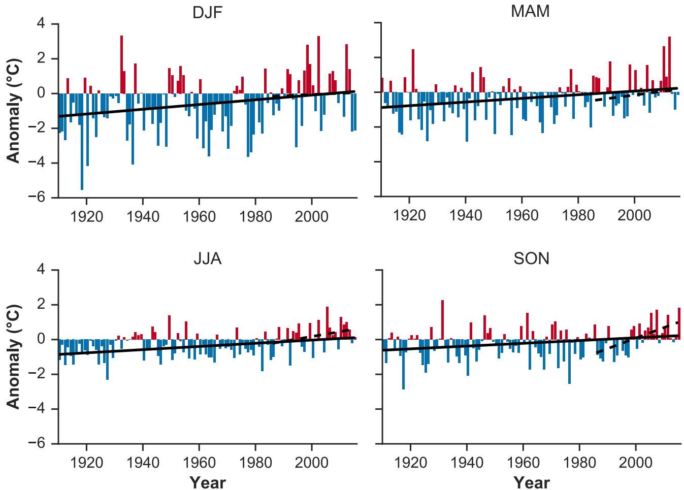
Figure 7.1.3 Anomalies (with respect to the 1981–2010 average) of seasonal-mean temperature for the upper portion of the DRB. The solid and dashed lines are linear trends for the 1910–2015 and 1986–2015 periods, respectively.
