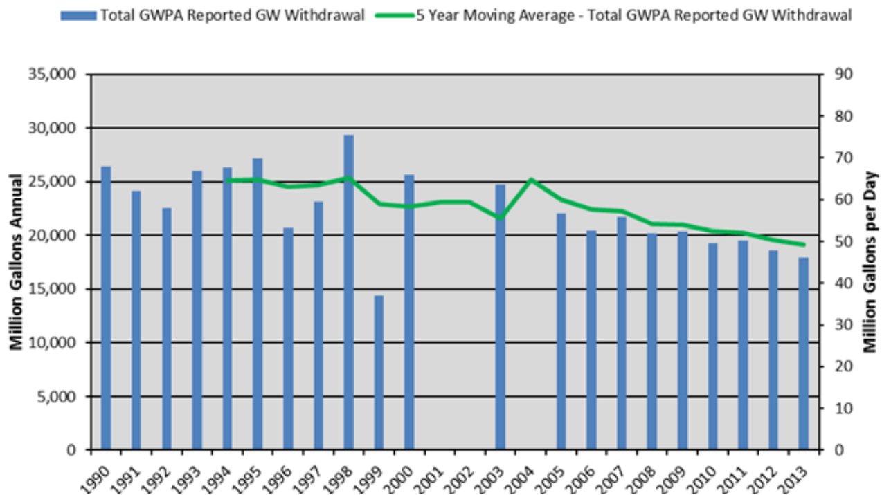
Figure 2.4.2 Groundwater withdrawals in the PA groundwater protected area 1990-2013.
