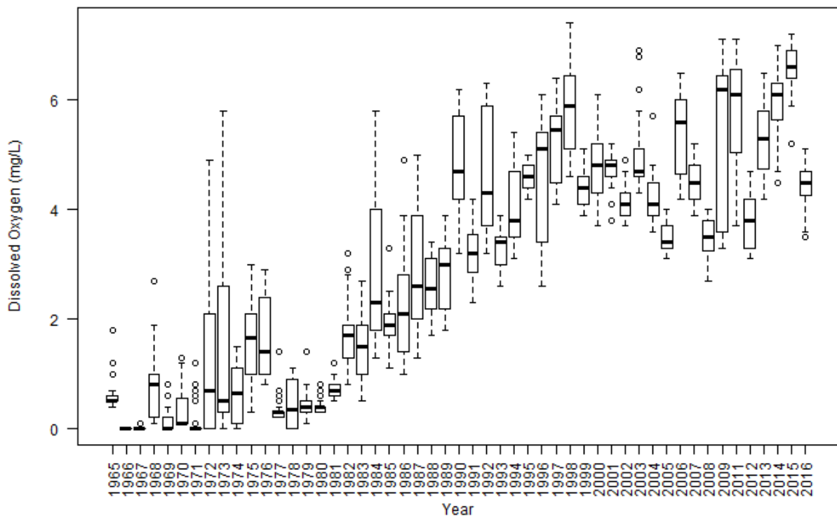
Figure 3.1.4 Delaware Estuary July daily minimum dissolved oxygen concentrations by year at USGS at Ben Franklin Bridge, 1965 through 2016.
