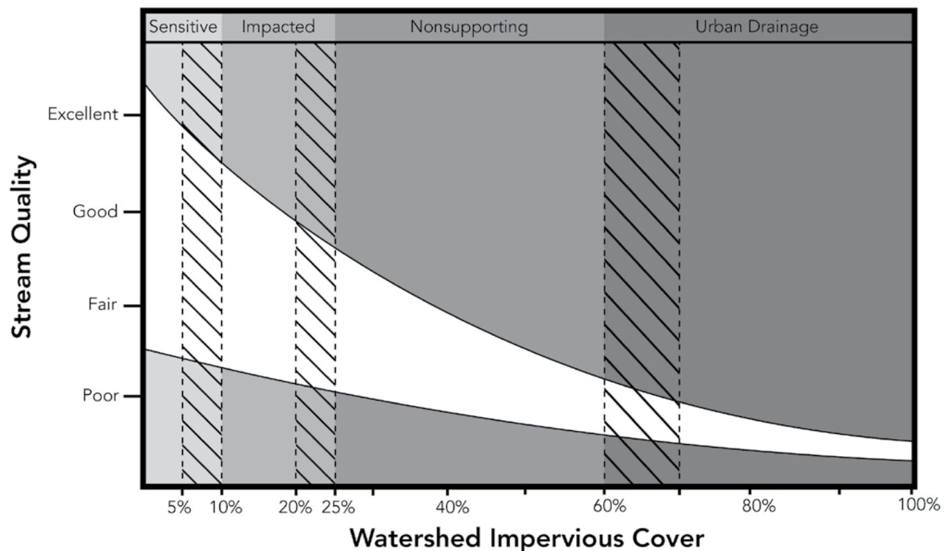
Figure 1.4.1 Center for Watershed Protection’s model of impervious cover impacts on streams.
