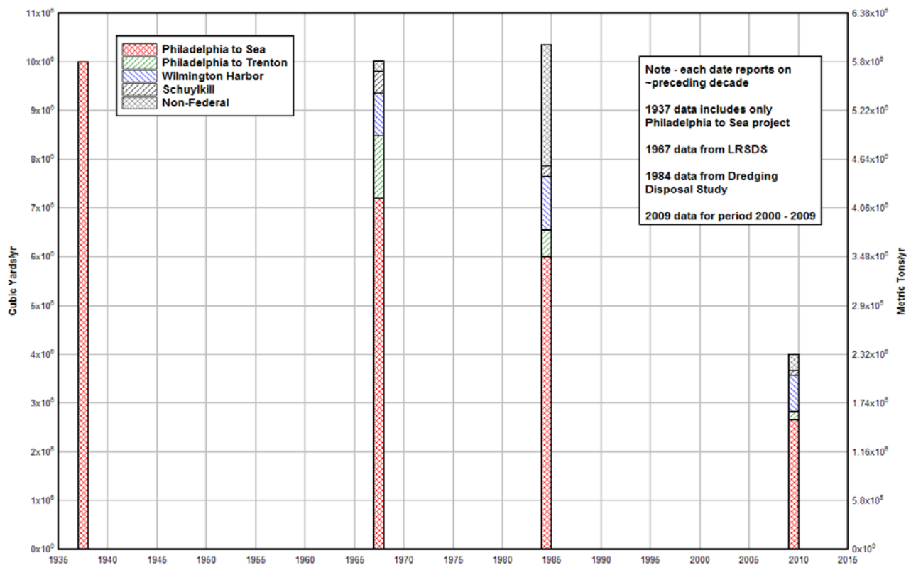
Figure 4.5.2 Average annual maintenance dredging rates within the Delaware Estuary in 1937, 1967, 1984, and 2009.
